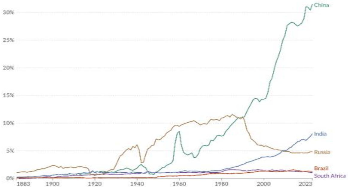
Figure 2: Global Share of BRICS in CO 2 Emissions
